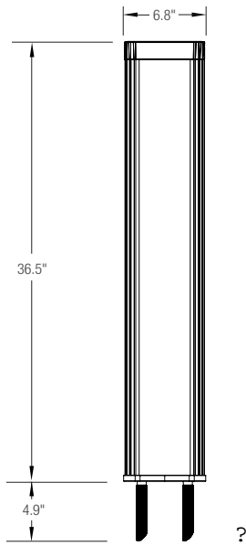
SOLAR BOLLARD
